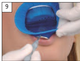
9. Position the dam in the lower vestibular region. Einsetzen ins untere Vestibulum.
